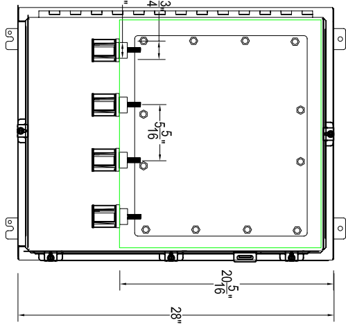
1 FRONT VIEW W0800-21-2228-1
