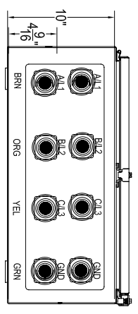
1 BOTTOM VIEW W0800-21-2228-1
