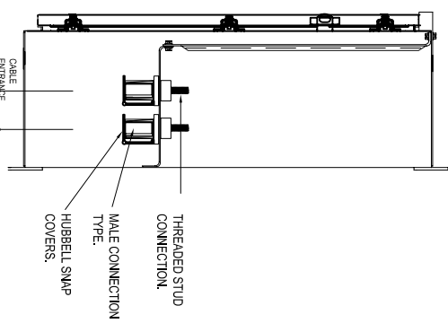
1 SIDE VIEW W0800-21-2228-1
