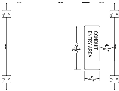
1 BACK VIEW W0800-21-2228-1
